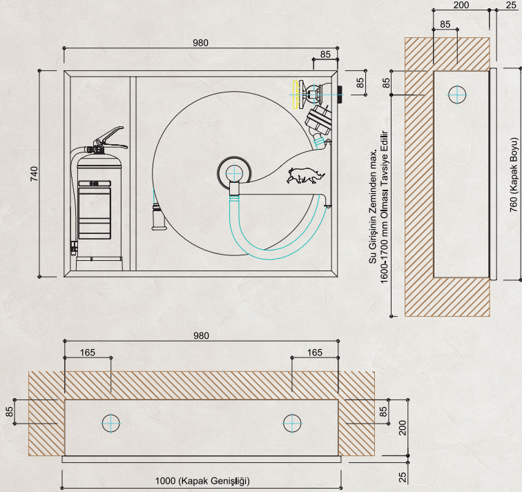
GÖMME TİP
